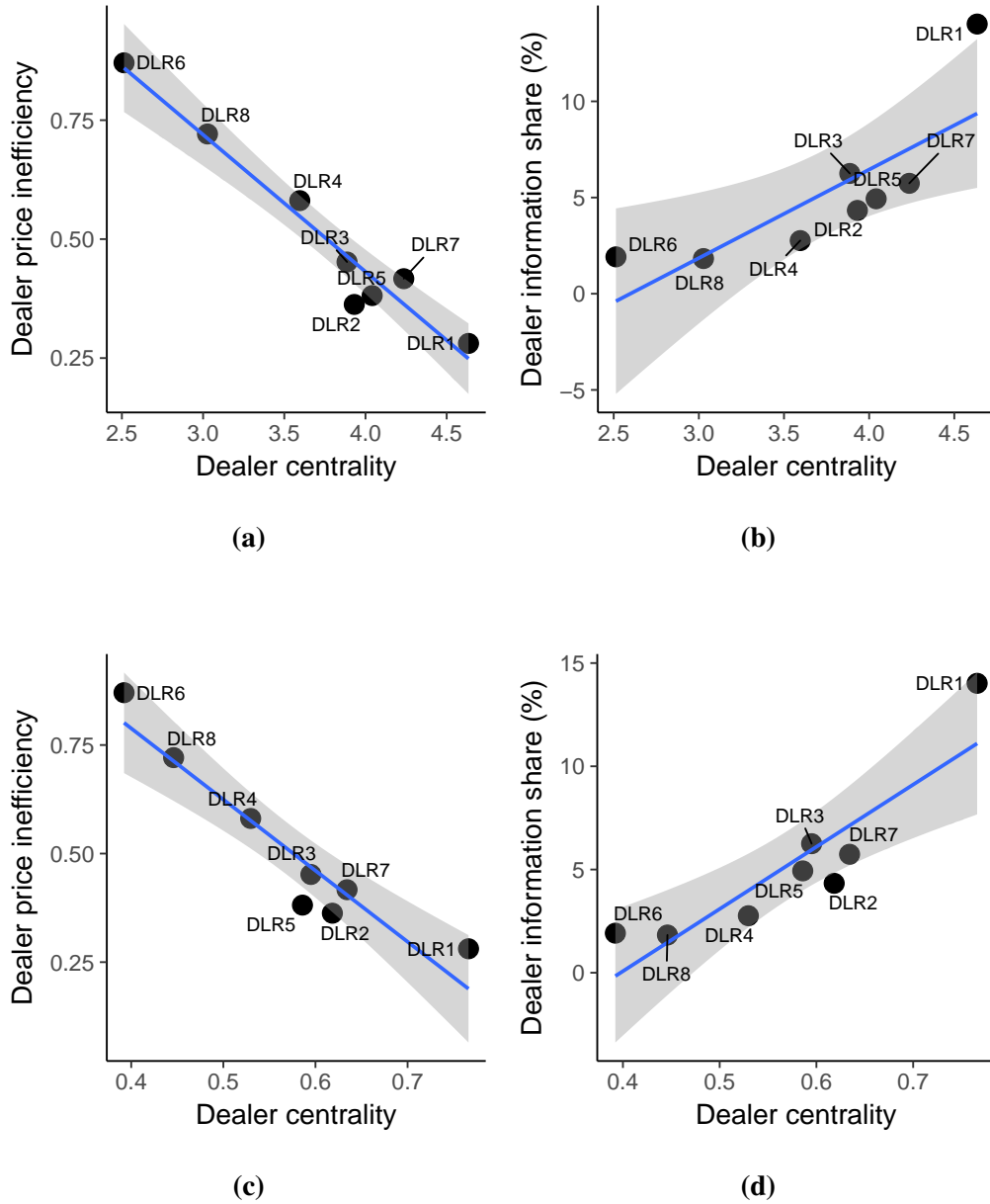
Figure IA.4: Scatter plot of a dealer centrality versus price informativeness. This figure replicates Figure 4 using alternative centrality measures. Panels (a) and (b) use Centrality0.1 , and Panels (c) and (d) use CentralityAll .
