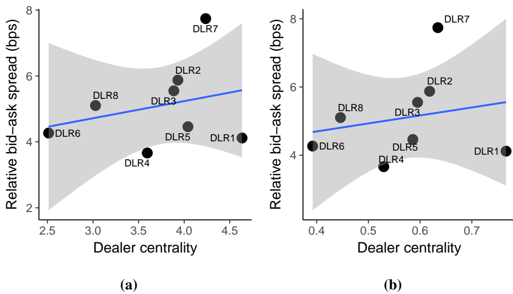
Figure IA.5: Scatter plot of dealer centrality versus quoted bid-ask spread. This figure replicates Figure 5 using alternative centrality measures. Panel (a) uses Centrality0.1 , and Panel (b) uses CentralityAll .
